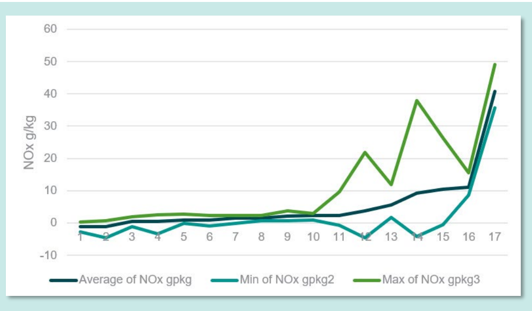
Figure 66: NO x emissions for HDV seen more than 4 times—model year 2010 and newer
