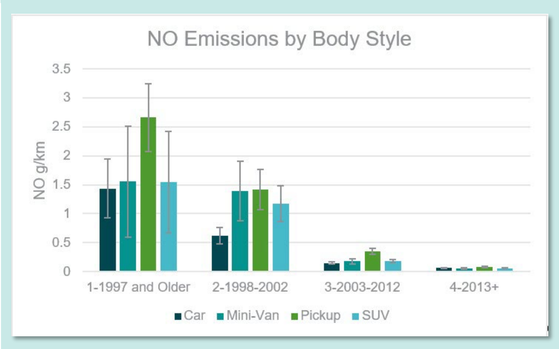
Figure 45: LDV NO emissions by body style
