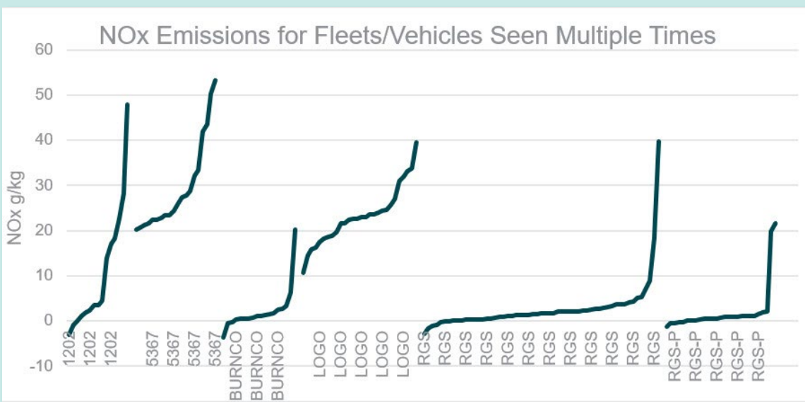
Figure 68: HDV NO x emissions for fleets/vehicles seen multiple times
