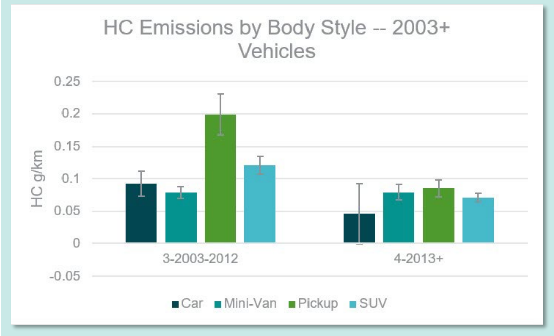
Figure 44: LDV HC emissions by body style, vehicles 2003 and newer
