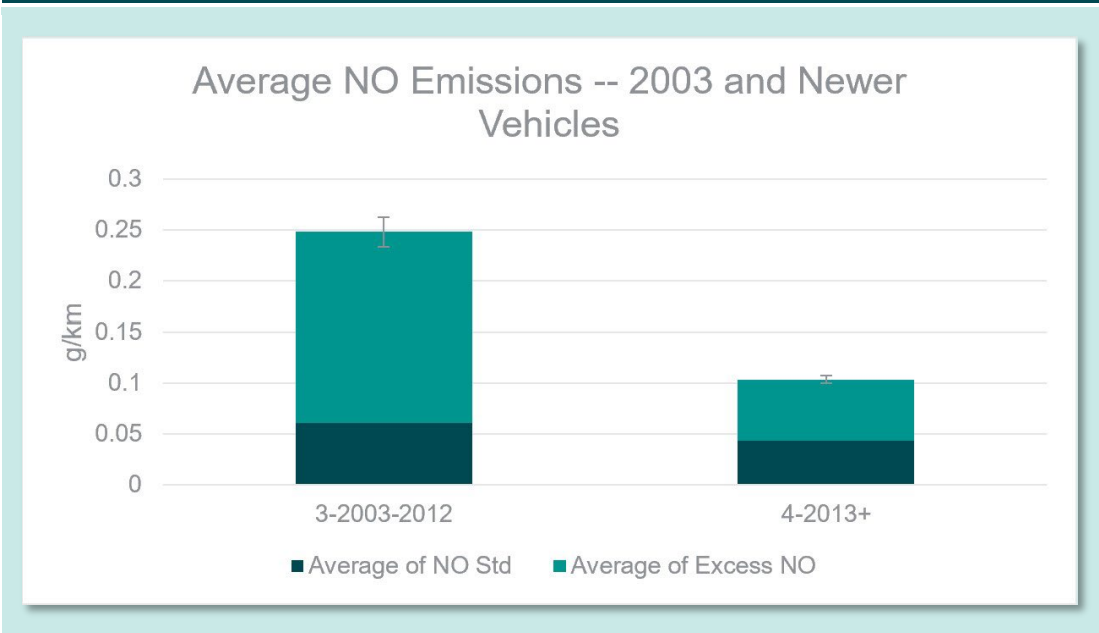
Figure 32: Average NO emissions—LDV model year 2003 and newer
