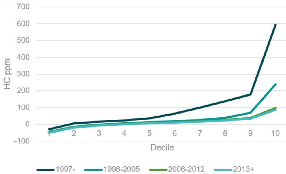
Figure 77: HC Emission Deciles—LDVs
