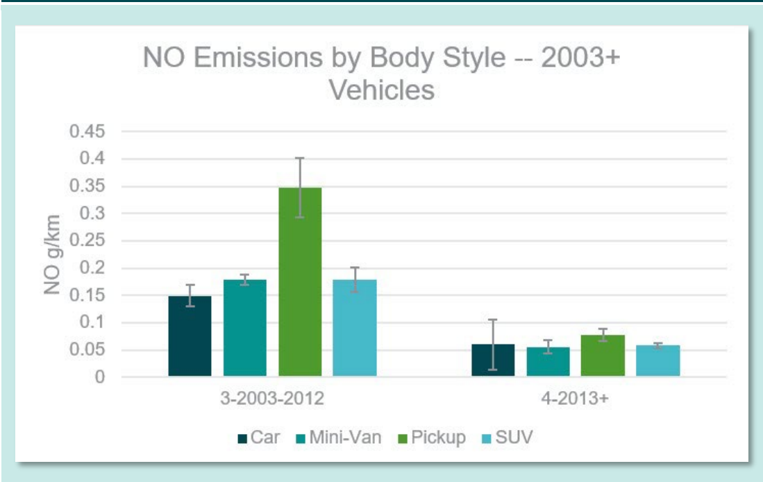
Figure 46: LDV NO emissions by body style, vehicles 2003 and newer
