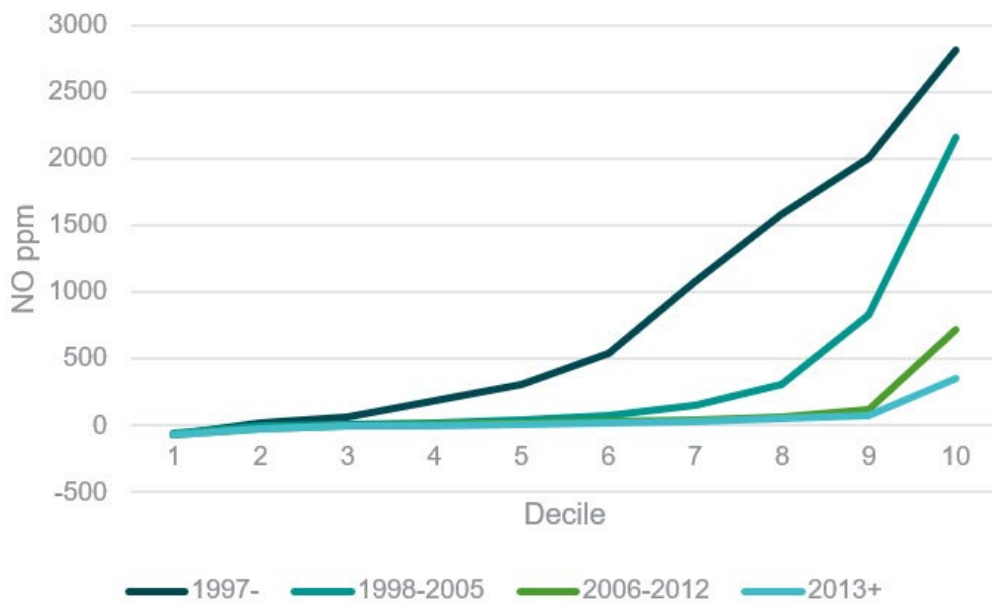
Figure 78: NO Emission Deciles—LDVs
