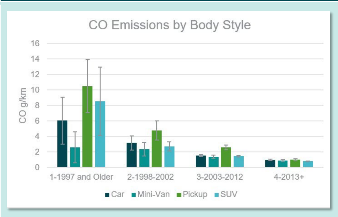
Figure 42: LDV CO emissions by body style
