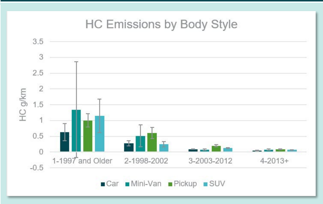
Figure 43: LDV HC emissions by body style
