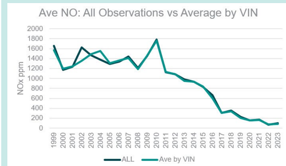
Figure 72: Average NO heavy-duty vehicles—All observations vs average by VIN
