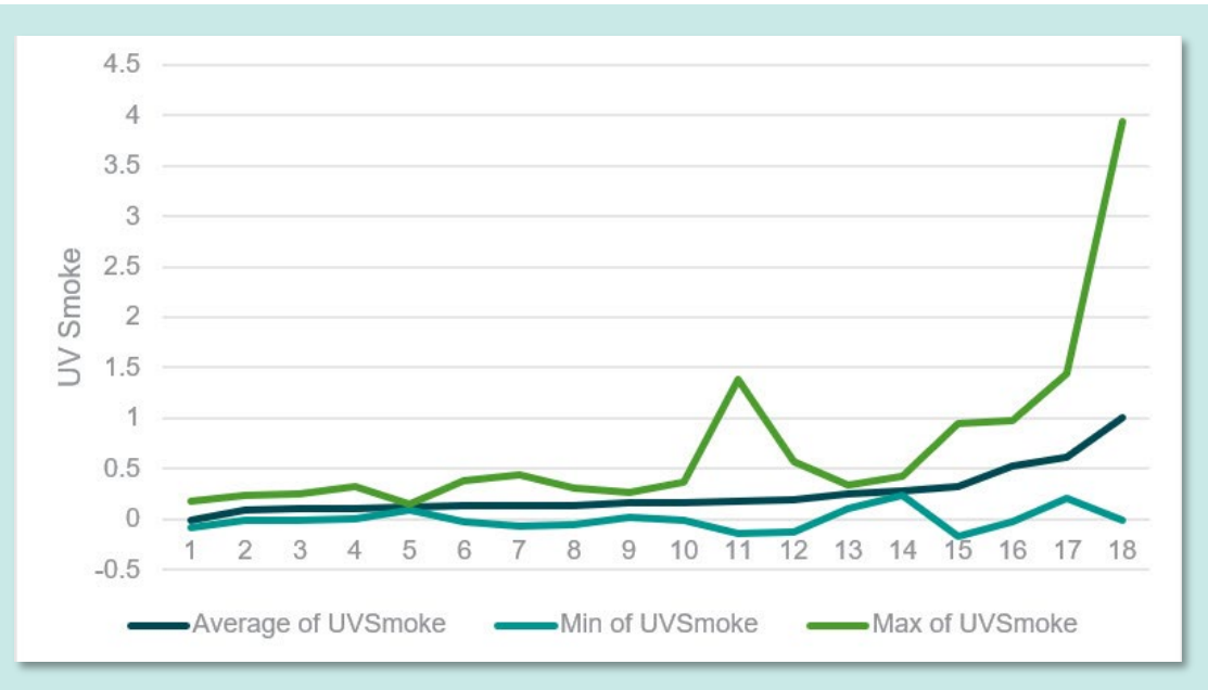
Figure 67: UV smoke emissions for HDV seen more than 4 times—model year 2010 and newer
