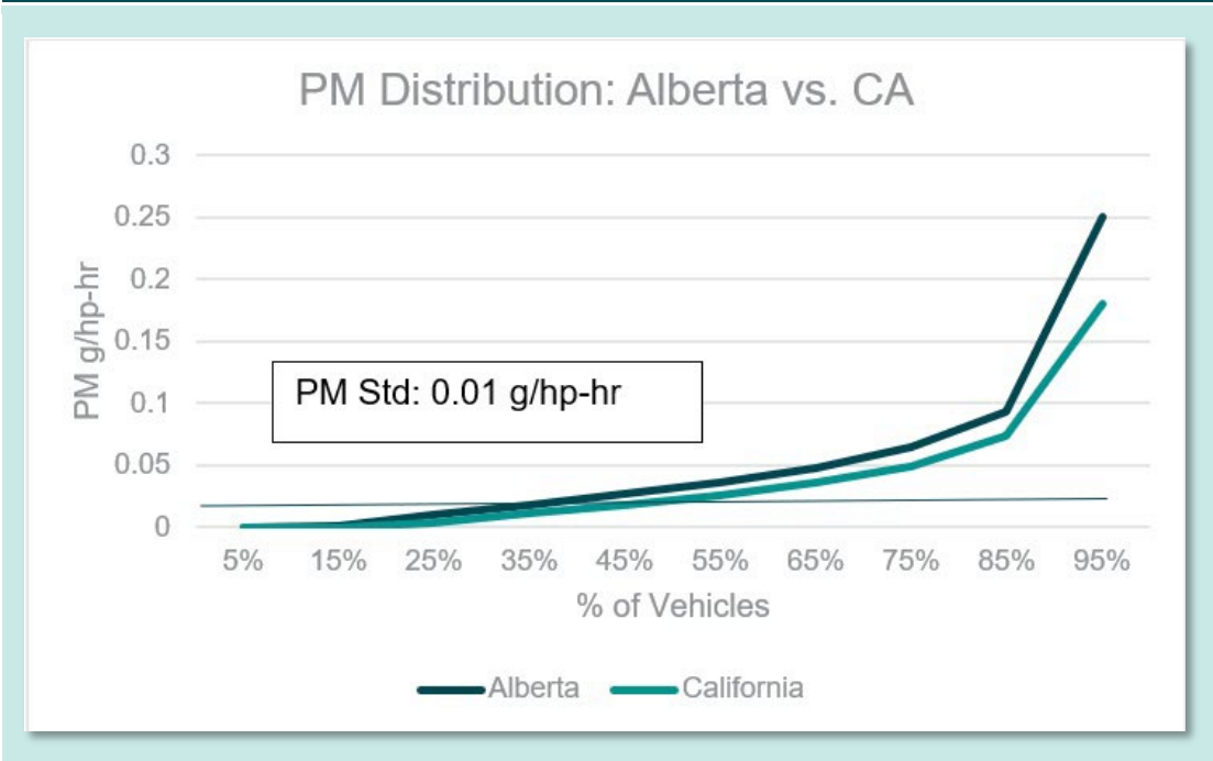
Figure 61: HDV PM distribution—Alberta vs. California
