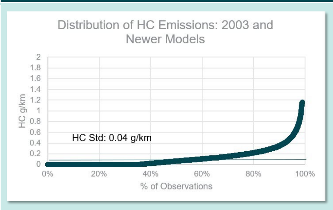
Figure 27: Distribution of HC emissions—2003 and newer LDV models
