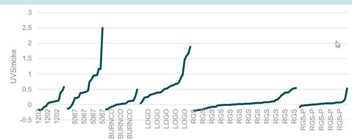
Figure 69: HDV UV smoke emissions for fleets/vehicles seen multiple times
