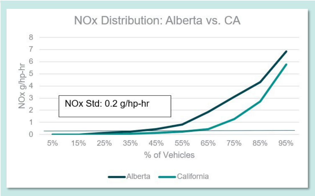
Figure 60: HDV NO x distribution—Alberta vs. California
