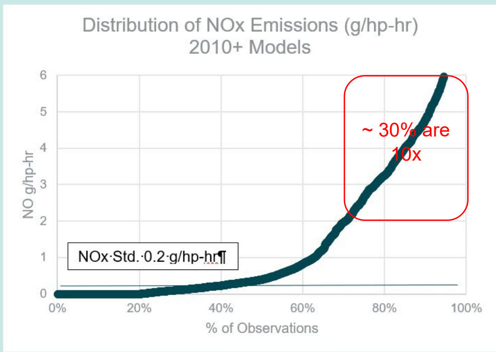
Figure 56: Distribution of HDV NO x emissions (g/hp-hr) 2010 and newer models
