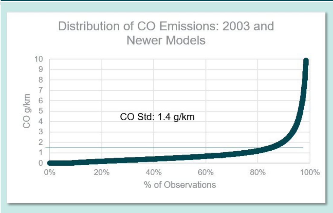
Figure 26: Distribution of CO emissions—2003 and newer LDV models
