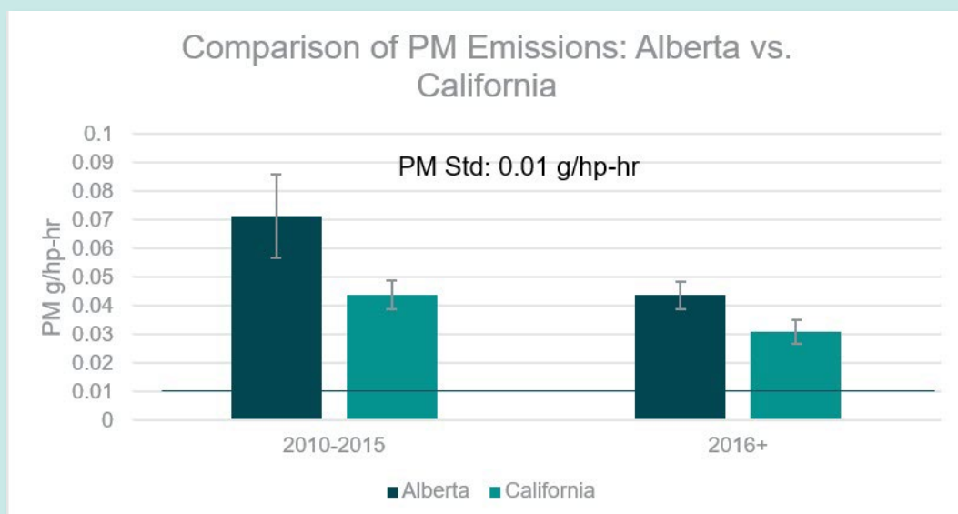
Figure 64: Comparison of HDV PM emissions—Alberta vs. California
