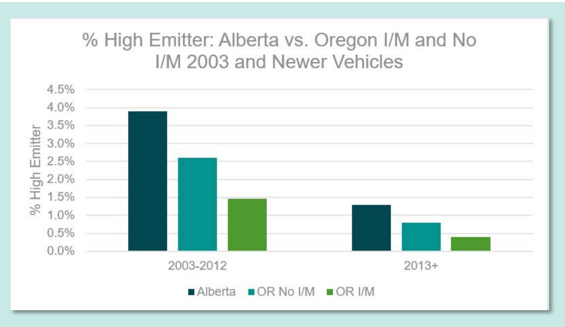
Figure 41: Percentage of LDV high emitters—Alberta vs. Oregon I/M and no-I/M, 2003 and newer vehicles
