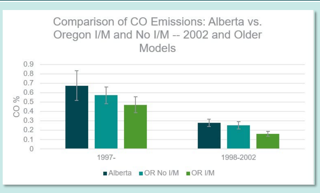
Figure 34: Comparison of LDV CO emissions—Alberta vs Oregon I/M and no-I/M, 2002 and older models
